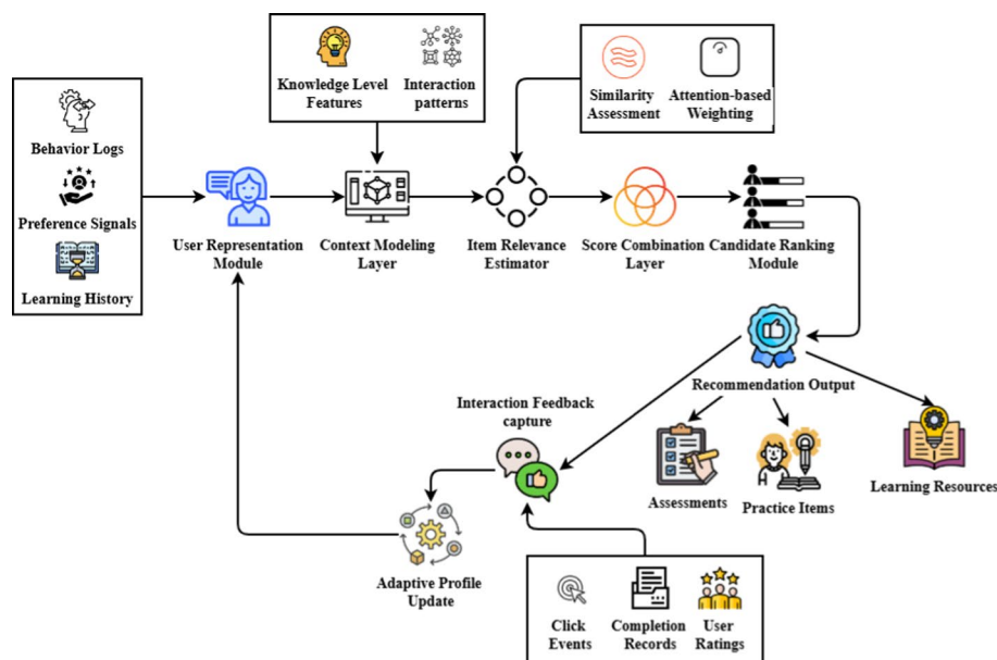
Fig. 4 Recommendation matching & scoring
